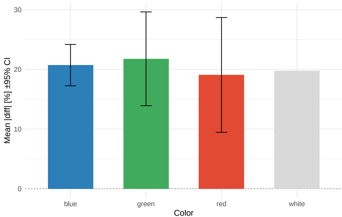
Rz1max effect by color Material/process: 14301_TR
