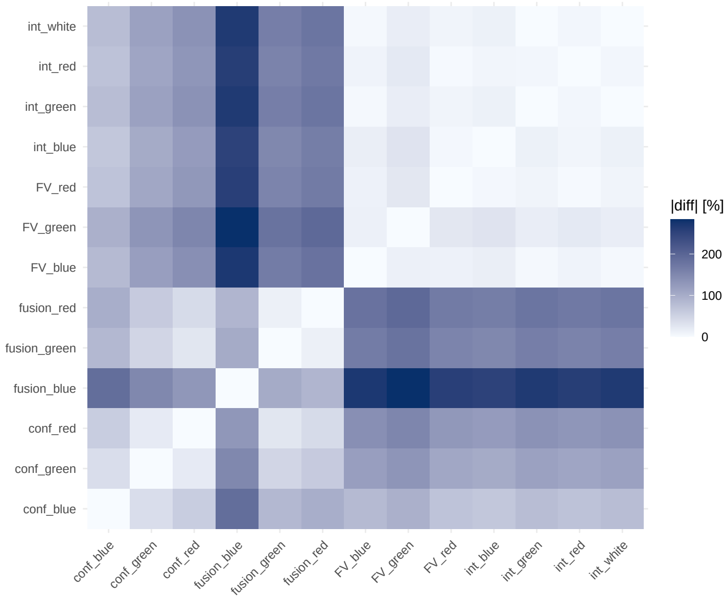
Material/process: C45_WEDM_F
