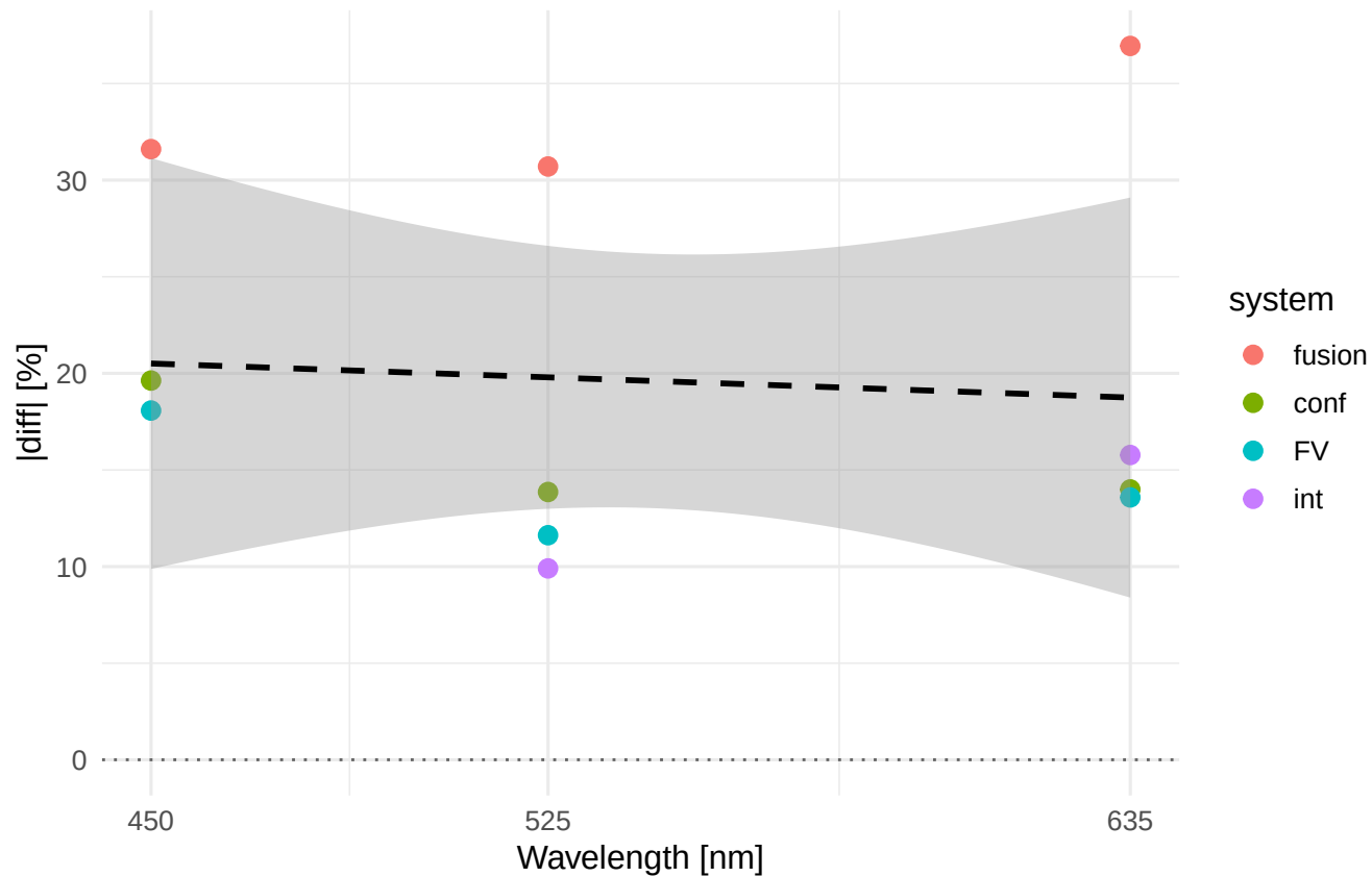
Rz1max |diff|% vs wavelength Material/process: ELLOR_WEDM_F
