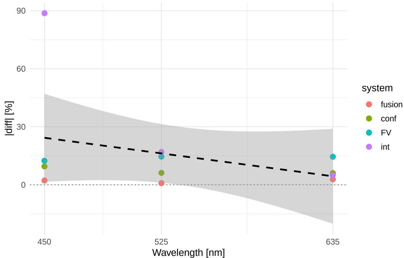
Rz1max |diff|% vs wavelength Material/process: ELLOR_WEDM_R
