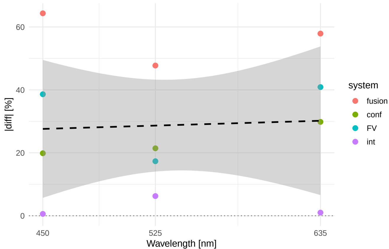
Rz |diff|% vs wavelength Material/process: 14301_GRI
