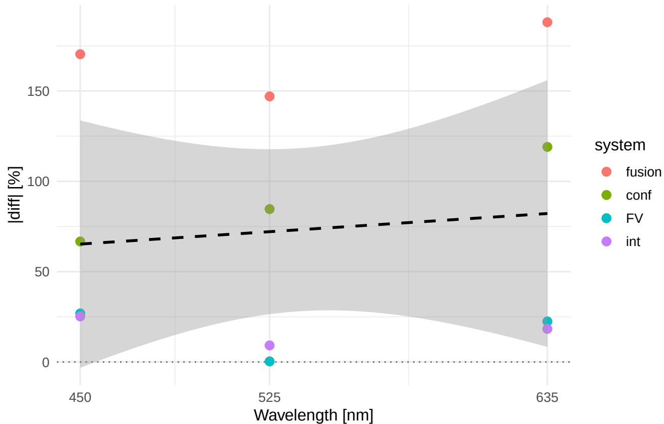
Rz |diff|% vs wavelength Material/process: 14301_WEDM_F
