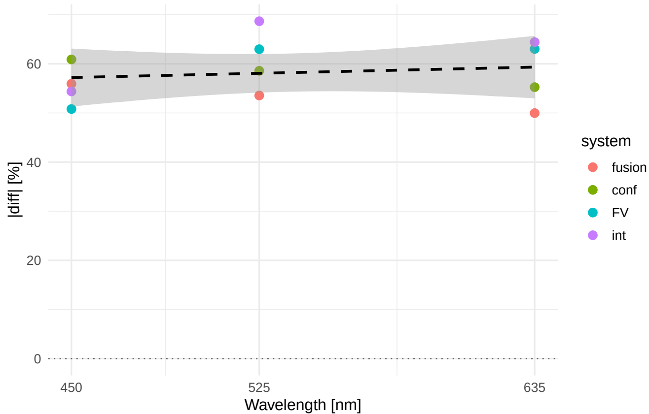
Rz |diff|% vs wavelength Material/process: Al7075_TR
