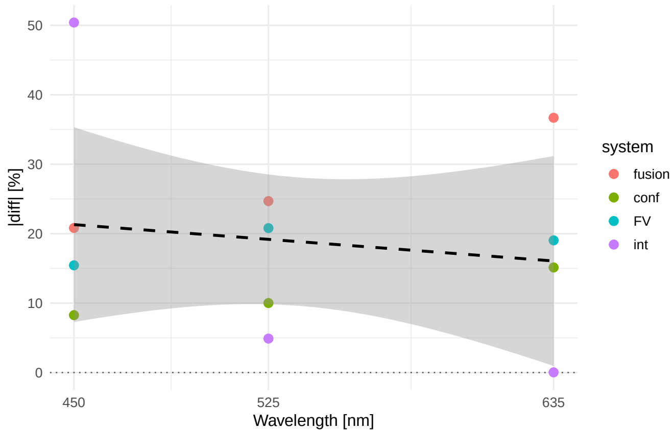
Rz |diff|% vs wavelength Material/process: ELLOR_TF
