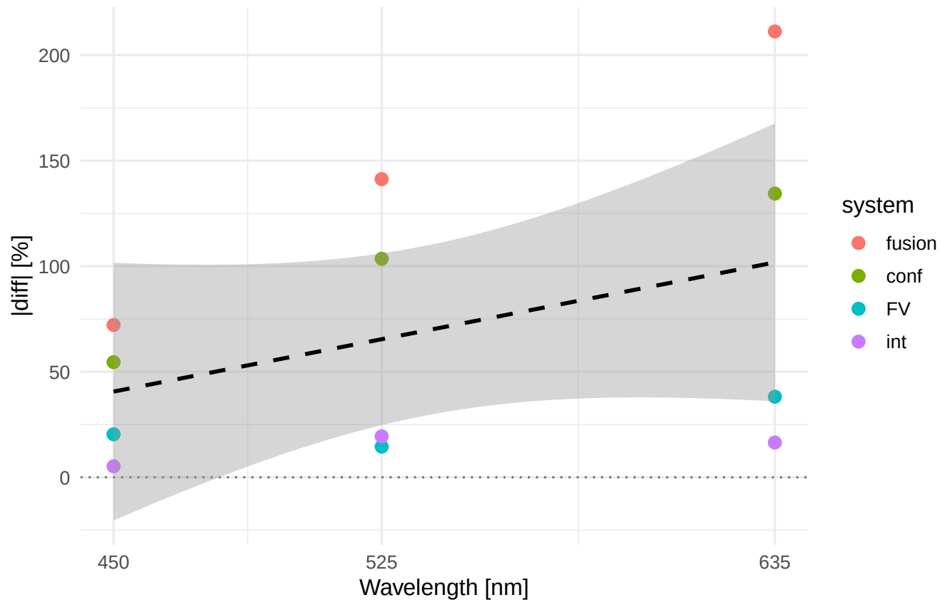
Rz |diff|% vs wavelength Material/process: MO58A_GLA
