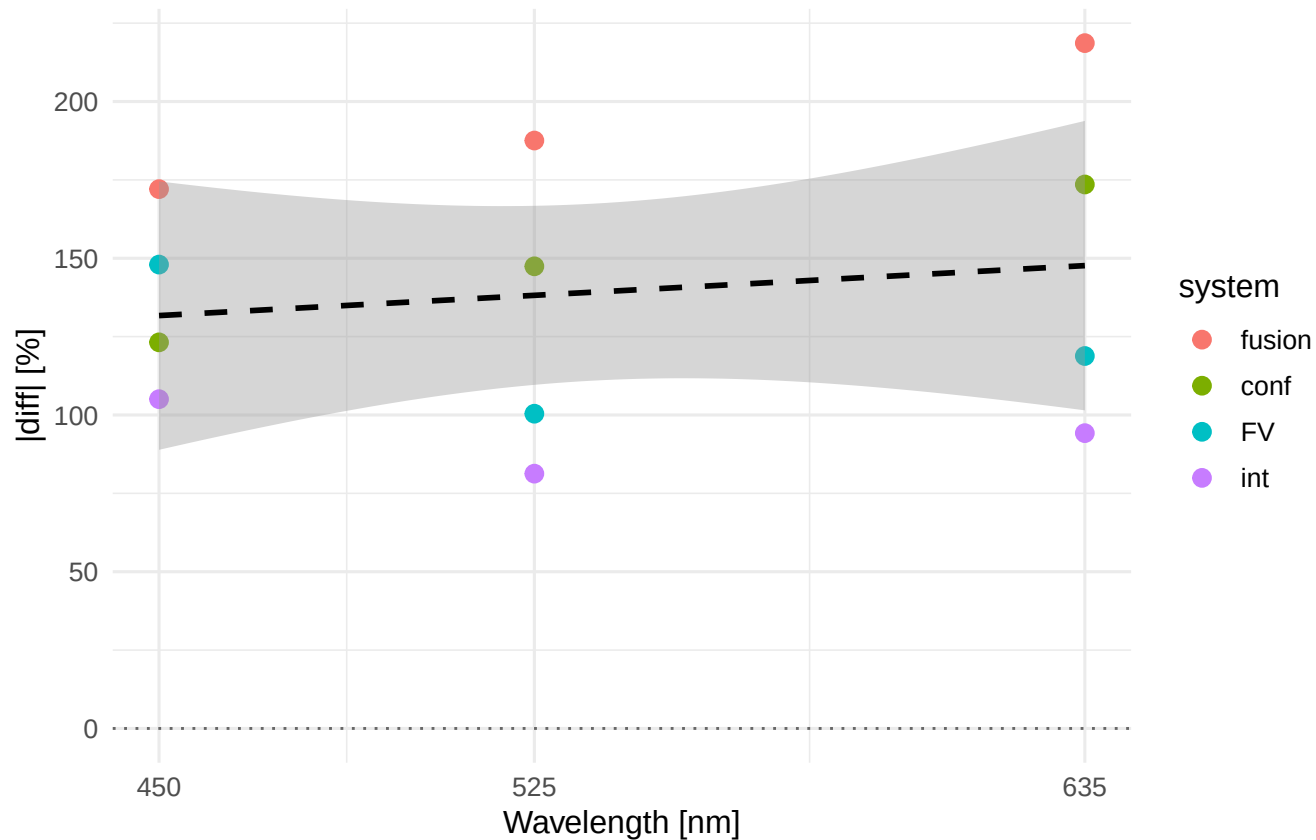
Rz |diff|% vs wavelength Material/process: Ti6Al4V_GRI
