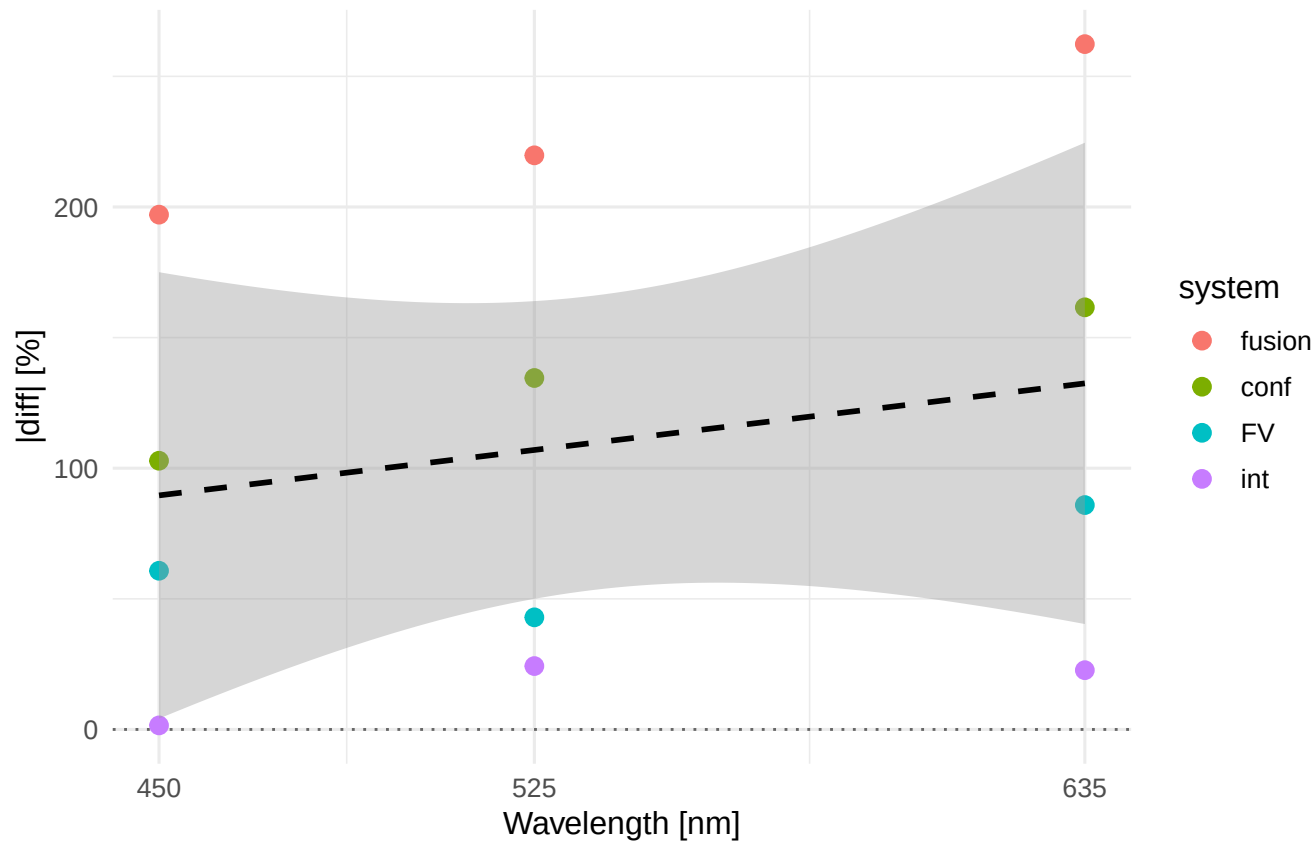
Rz |diff|% vs wavelength Material/process: Ti6Al4V_WEDM_F
