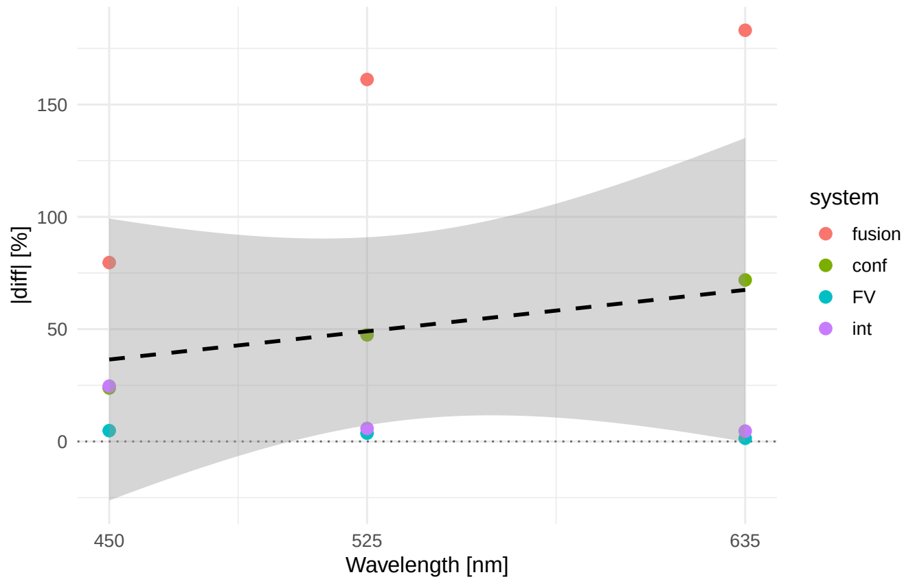
Rz |diff|% vs wavelength Material/process: Ti6Al4V_WEDM_R
