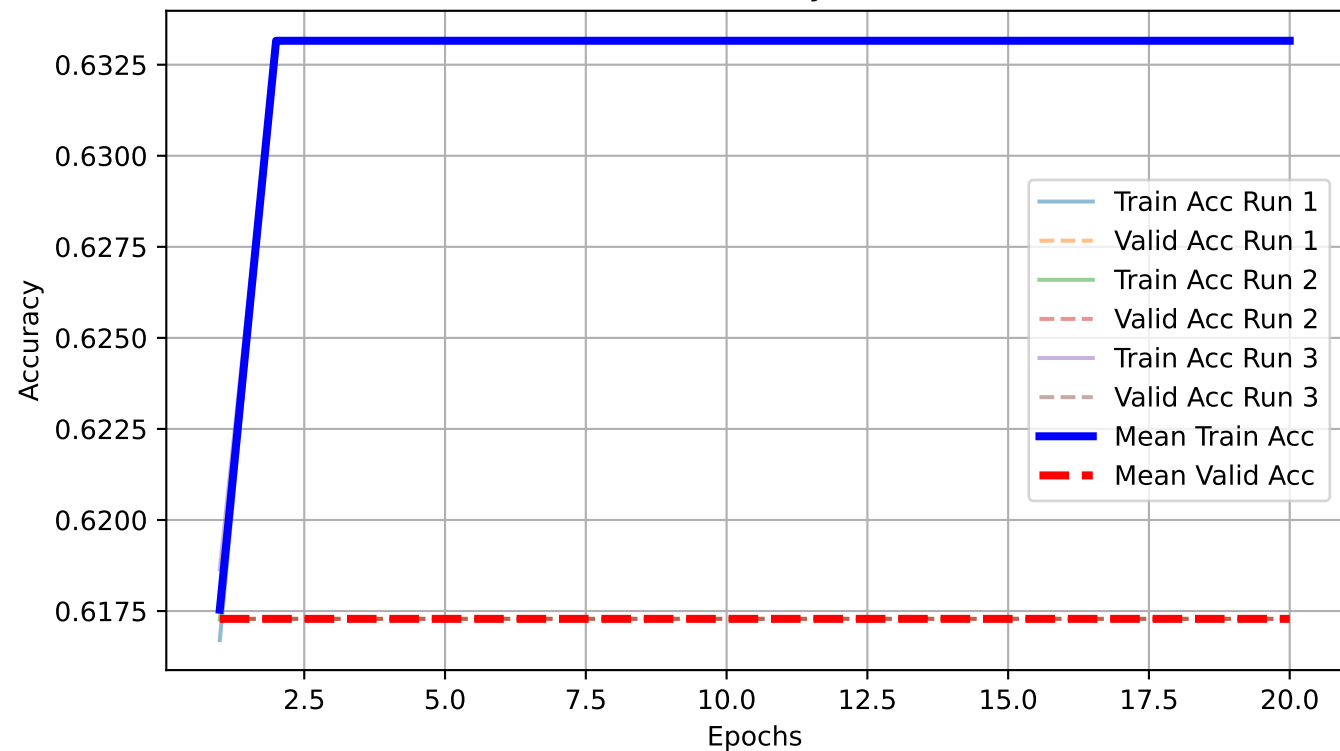
Accuracy
