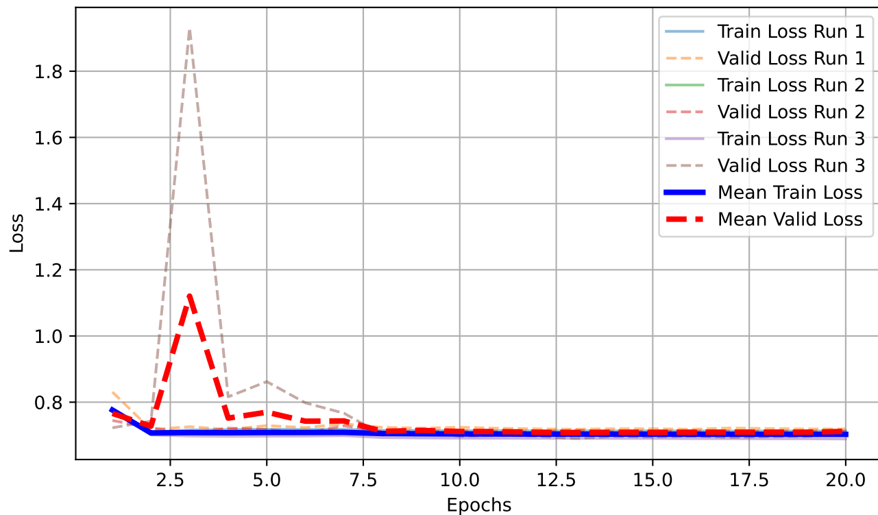
Loss
