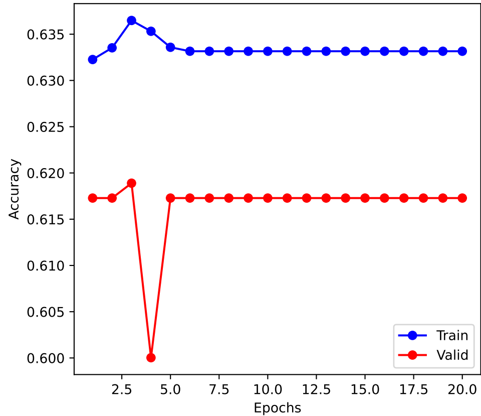
Accuracy
