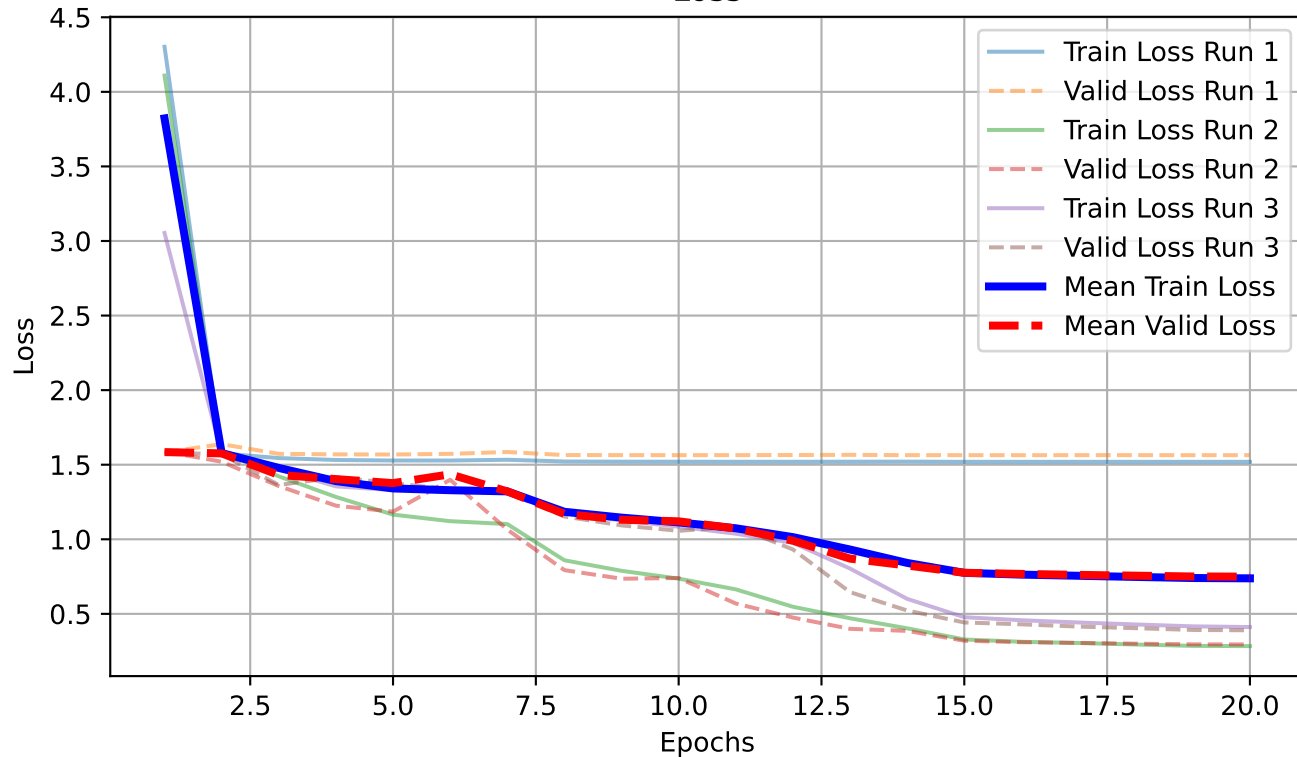
Loss
