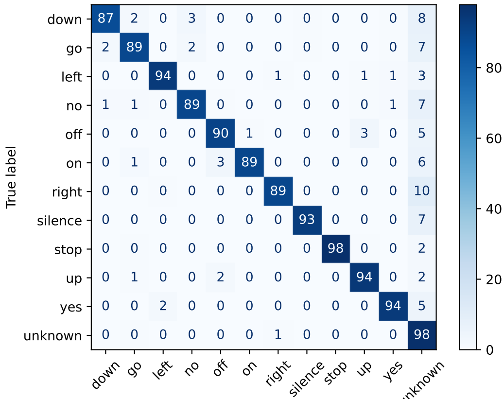
Normalized Confusion Matrix
