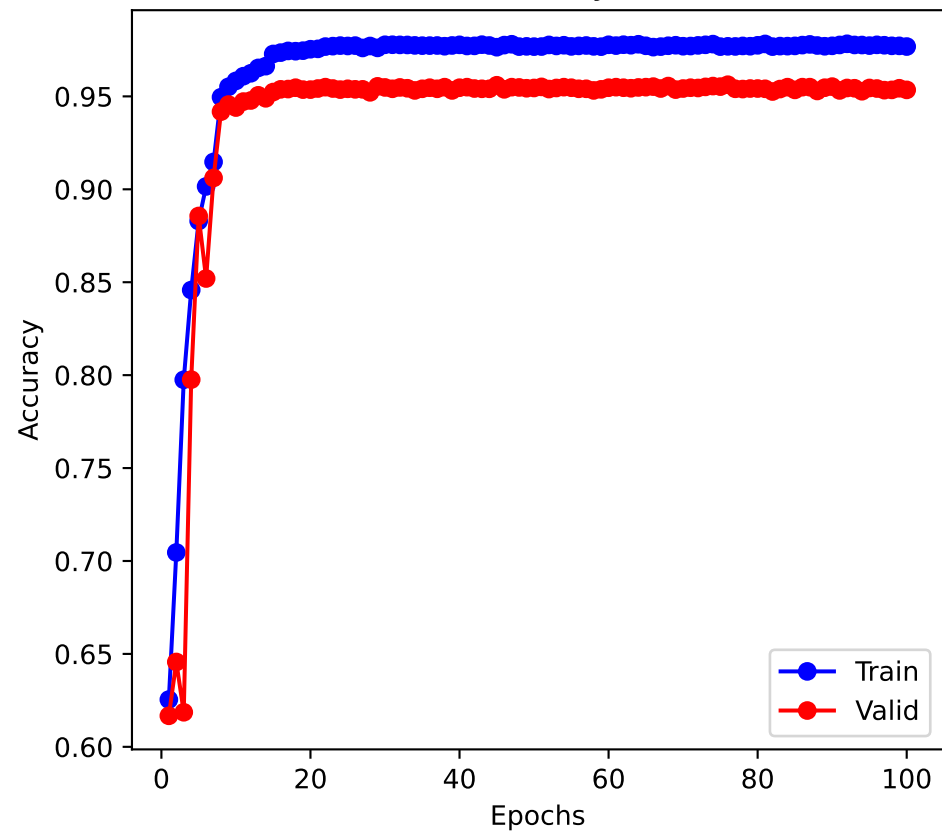
Accuracy
