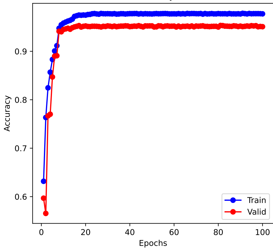
Accuracy
