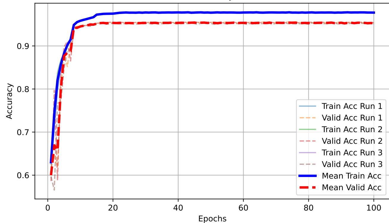
Accuracy
