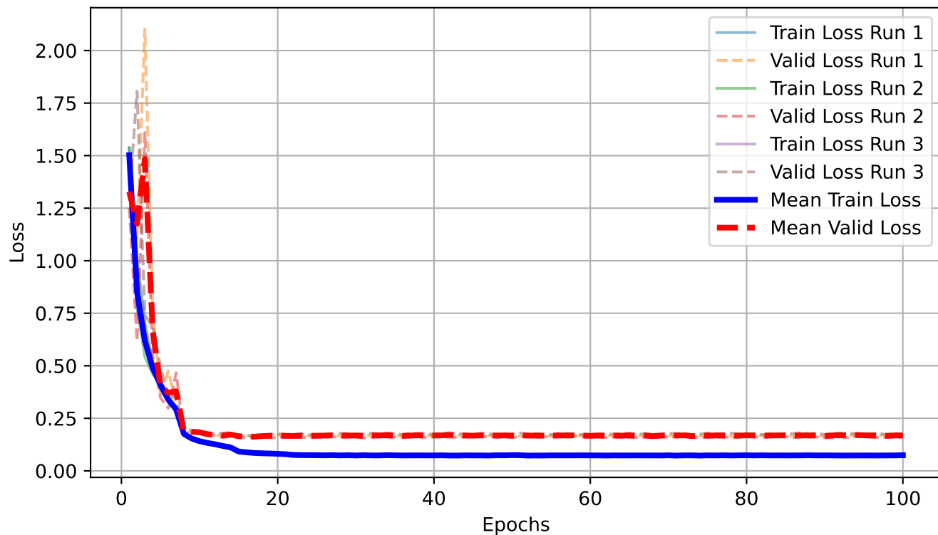
Loss
