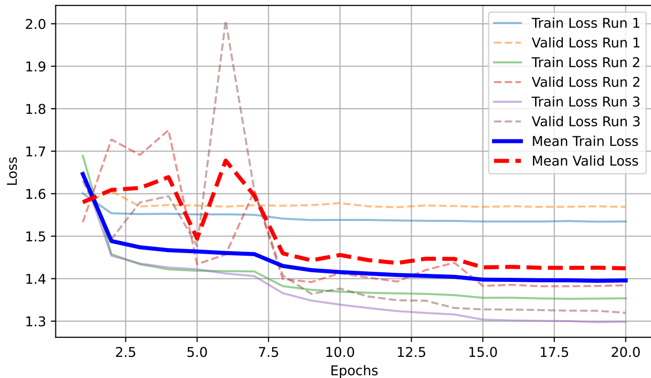
Loss
