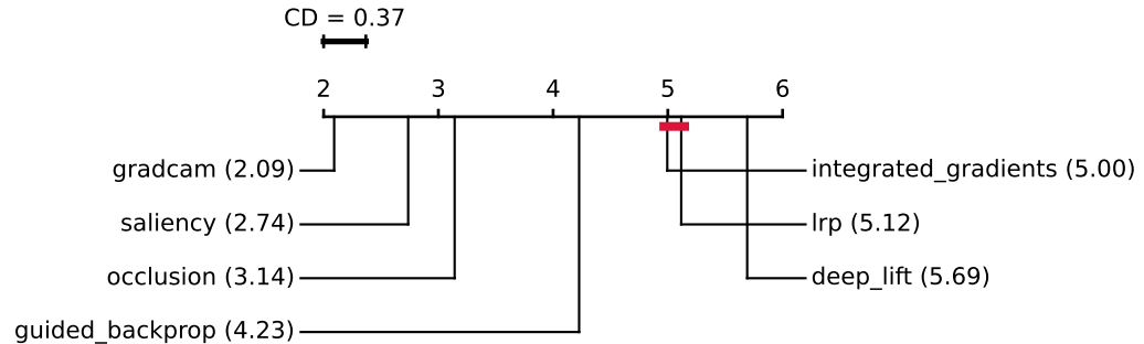
SqueezeNet (Autoweighted)
