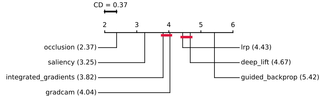
ResNet-18 (Autoweighted)
