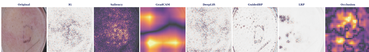
Fig. 1.1. Seven feature-attribution explanations of the same prediction (trained ResNet-18, dermoscopic test image ISIC_0012258 , melanoma class) from the ISIC 2017 dataset used in this thesis. The methods visibly disagree about which regions matter: the gradient-based methods (IG, Saliency, DeepLift, Guided Backpropagation, LRP) produce sharp but noisy pixel-level maps, while Grad-CAM and Occlusion yield coarse regional ones. Visual inspection cannot decide which of these is the better explanation of the model’s decision—quantifying that is the evaluation problem this thesis addresses.
