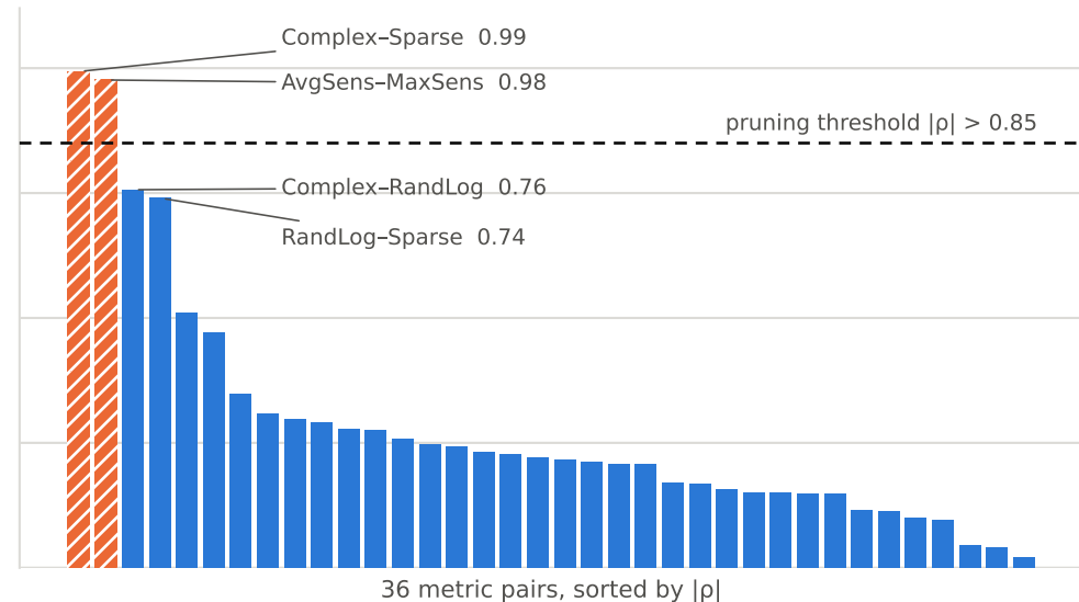
SqueezeNet
