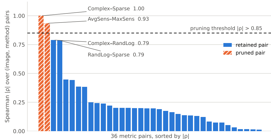
ResNet-18
