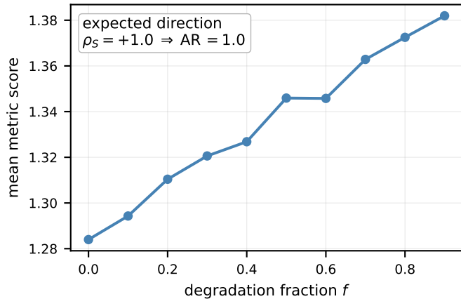
MaxSens / Integrated Gradients (ResNet-18)
