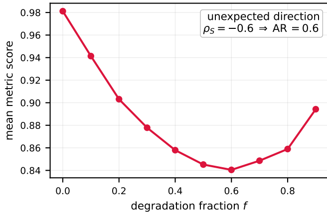
RandLog / Guided Backprop (ResNet-18)
