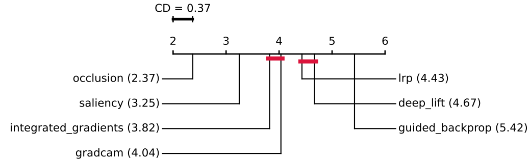
ResNet-18 (Autoweighted)
