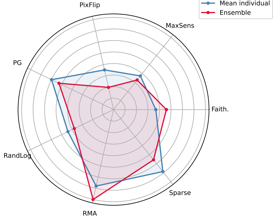
SqueezeNet
