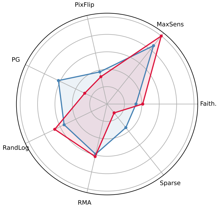
ResNet-18
