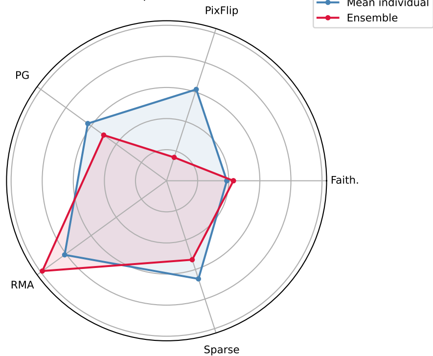
SqueezeNet
