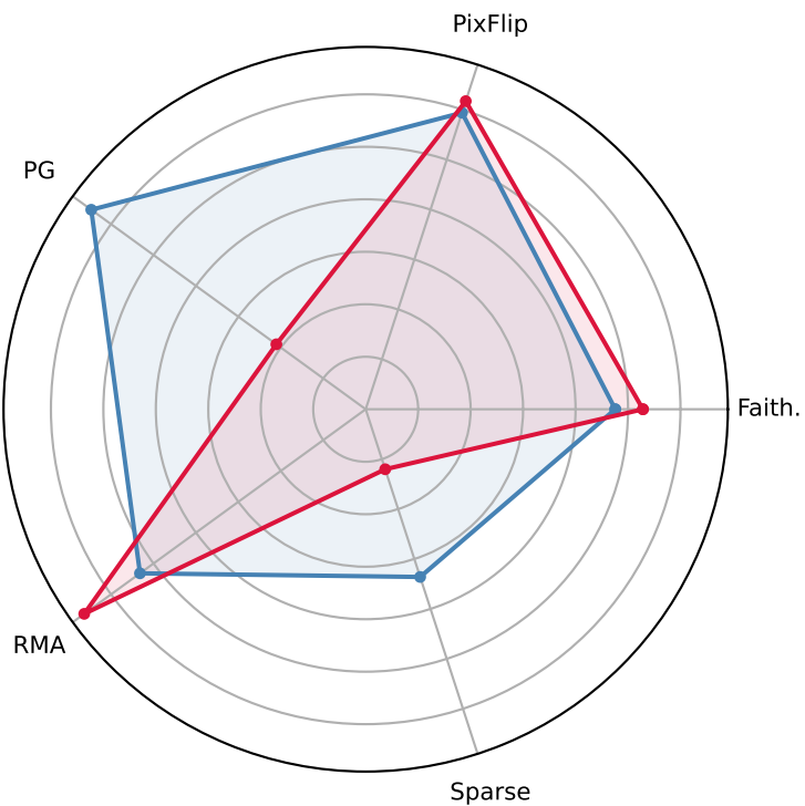
ResNet-18
