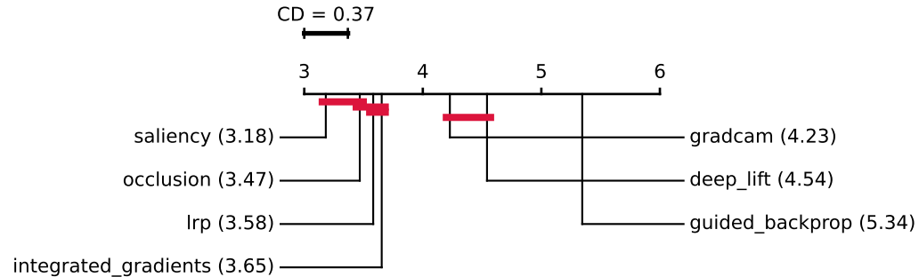
ResNet-18 (Autoweighted)
