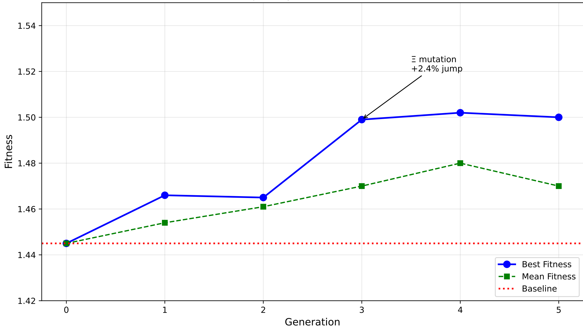
Evolution Trajectory: Fitness Over Generations
