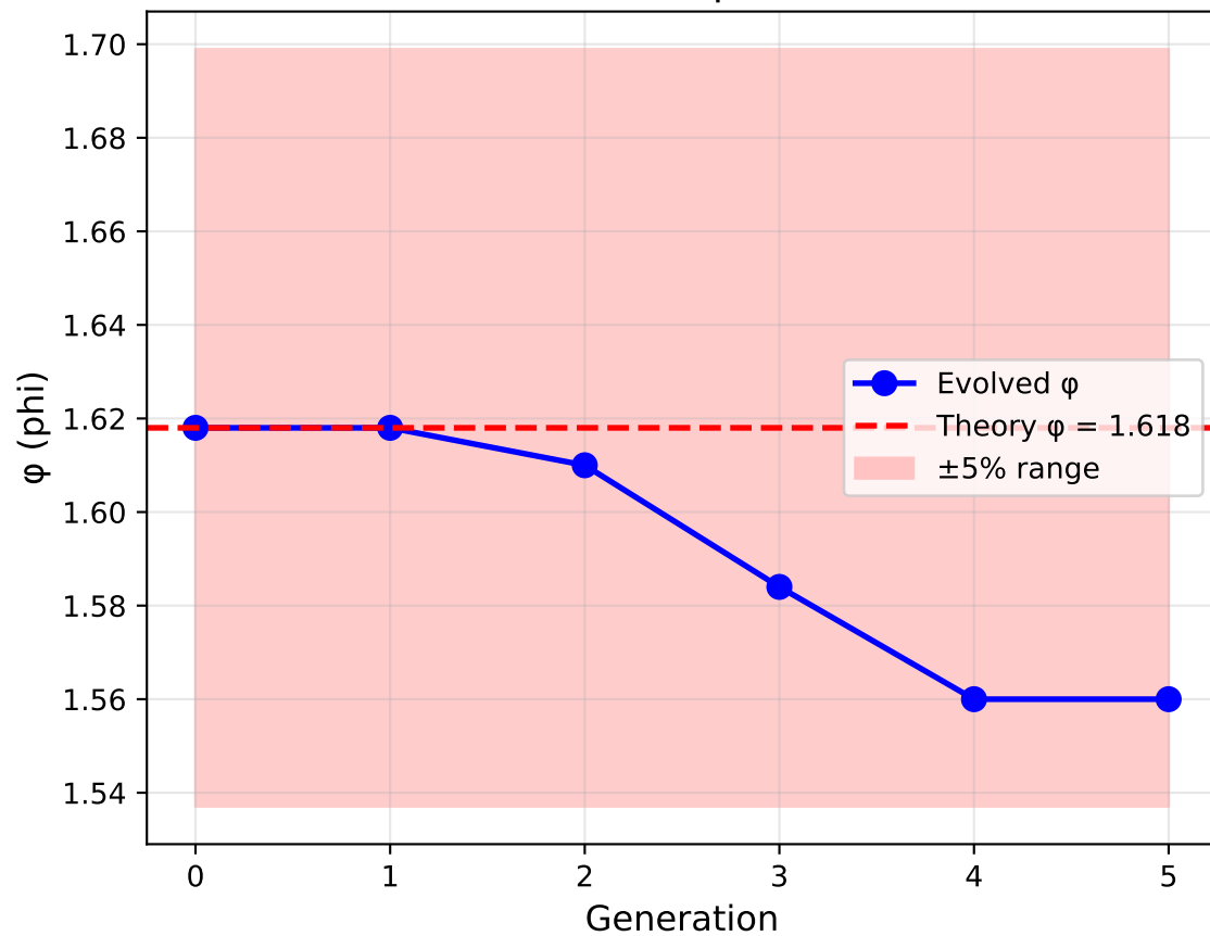
Golden Ratio ( \phi ) Evolution
