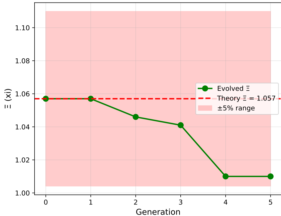
Balance Constant ( \Xi ) Evolution
