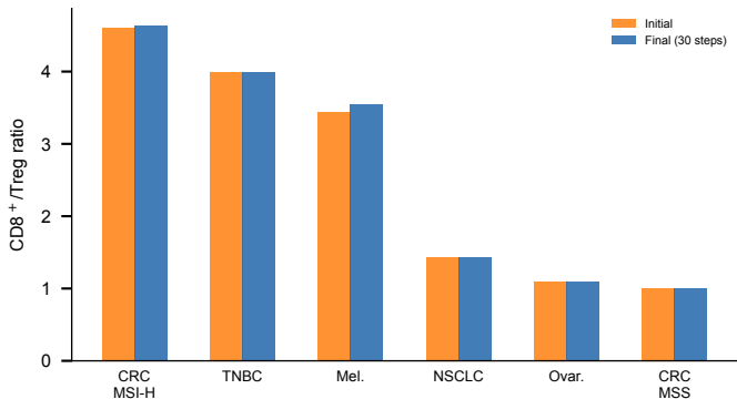
Figure S4: Initial vs final CD8/Treg across cancers
