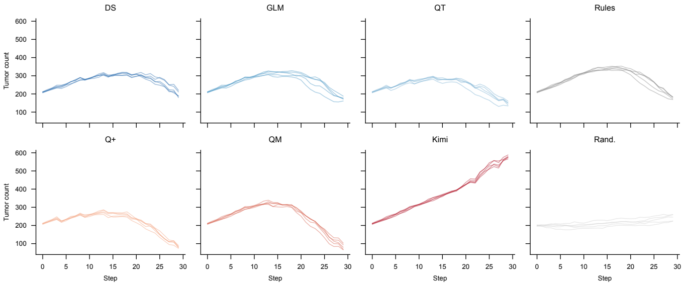
Figure S1: Individual tumor trajectories (5 seeds per model)
