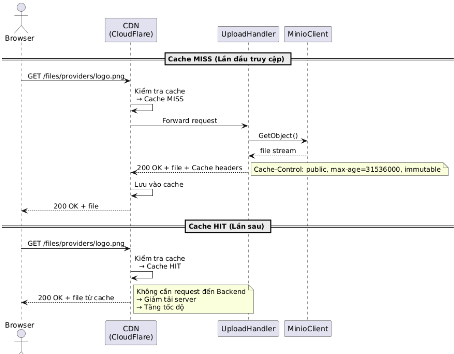
Sequence Diagram: CDN Caching Flow
