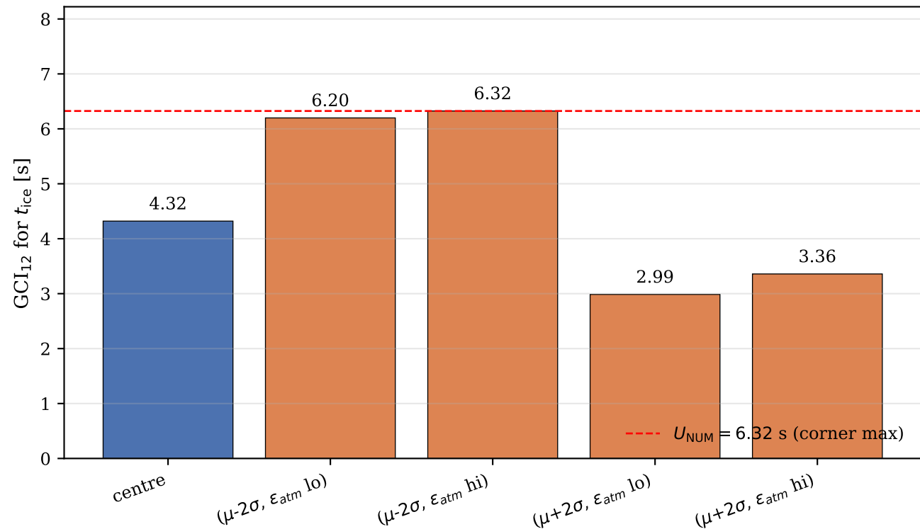
Numerical uncertainty across prediction-domain corners
