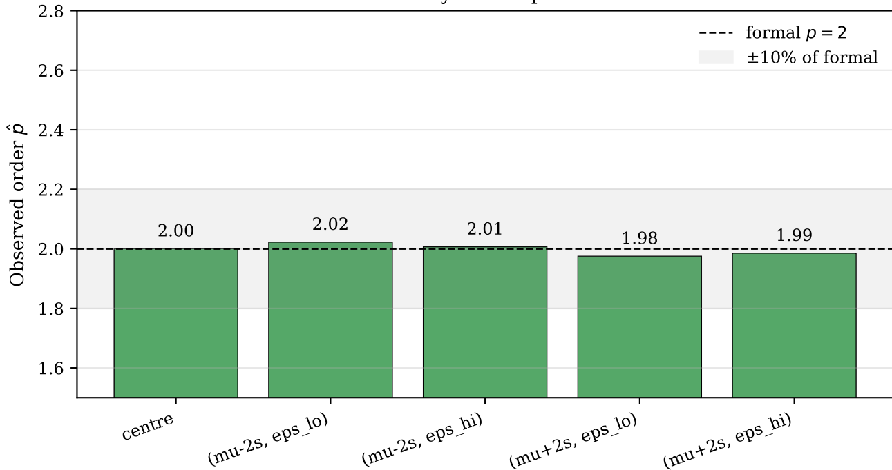
Observed order of accuracy across prediction-domain corners
