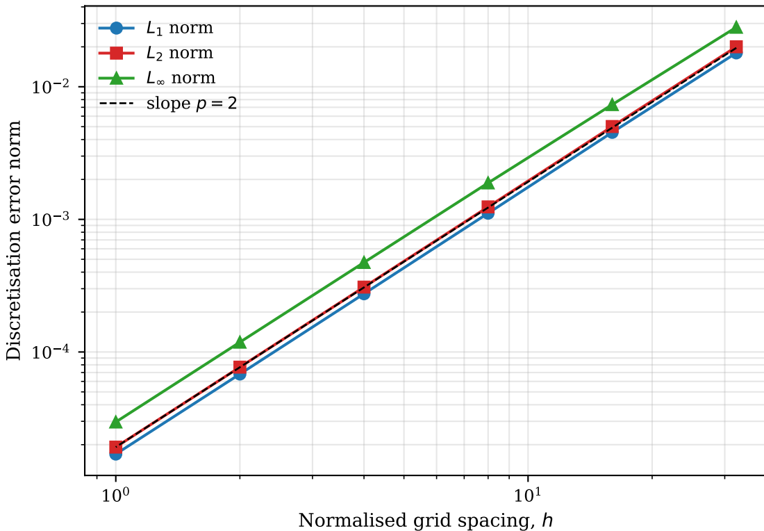
MMS code verification: error norms vs grid spacing
