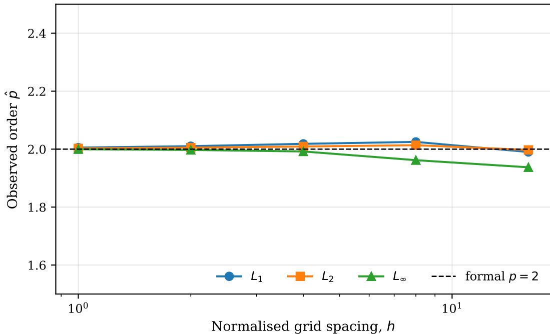
MMS: observed order of accuracy
