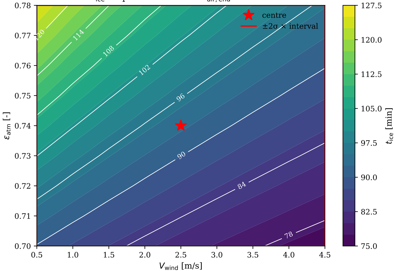
t_{\text{ice}} response surface at T_{\text{air, end}} = 263 \text{ K}
