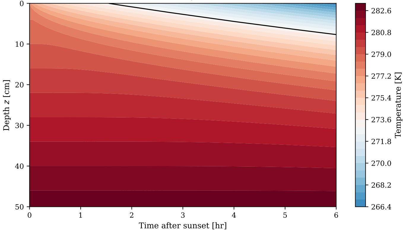
Road temperature field (prediction T_{\text{air, end}} = 263 \text{ K} ). Black contour = 0 \text{ }^{\circ}\text{C}
