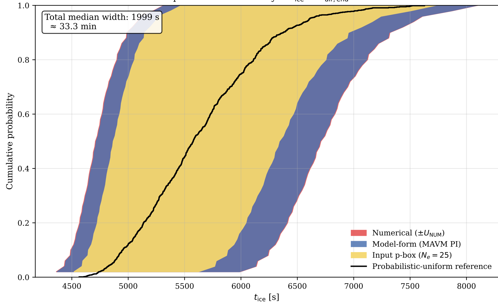
Total predictive uncertainty in t_{\text{ice}} at T_{\text{air, end}} = 263 \text{ K}
