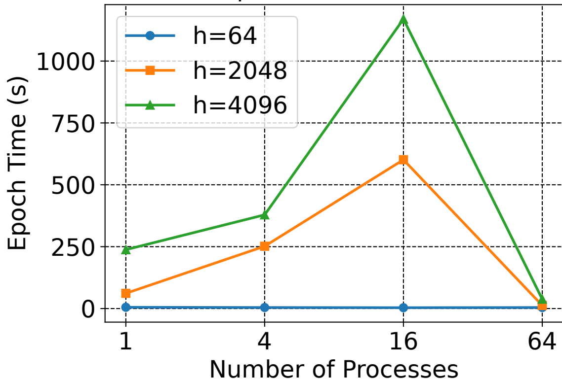
Mean Epoch Time vs Processes
