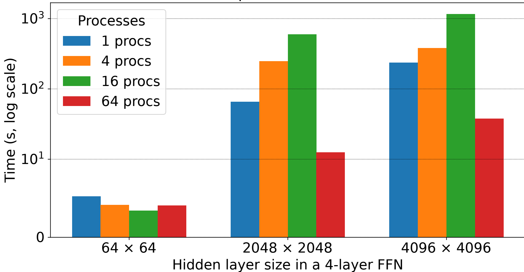
Mean Per Process Epoch Time Batches Per Epoch: 60, Batch Size: 1,000
