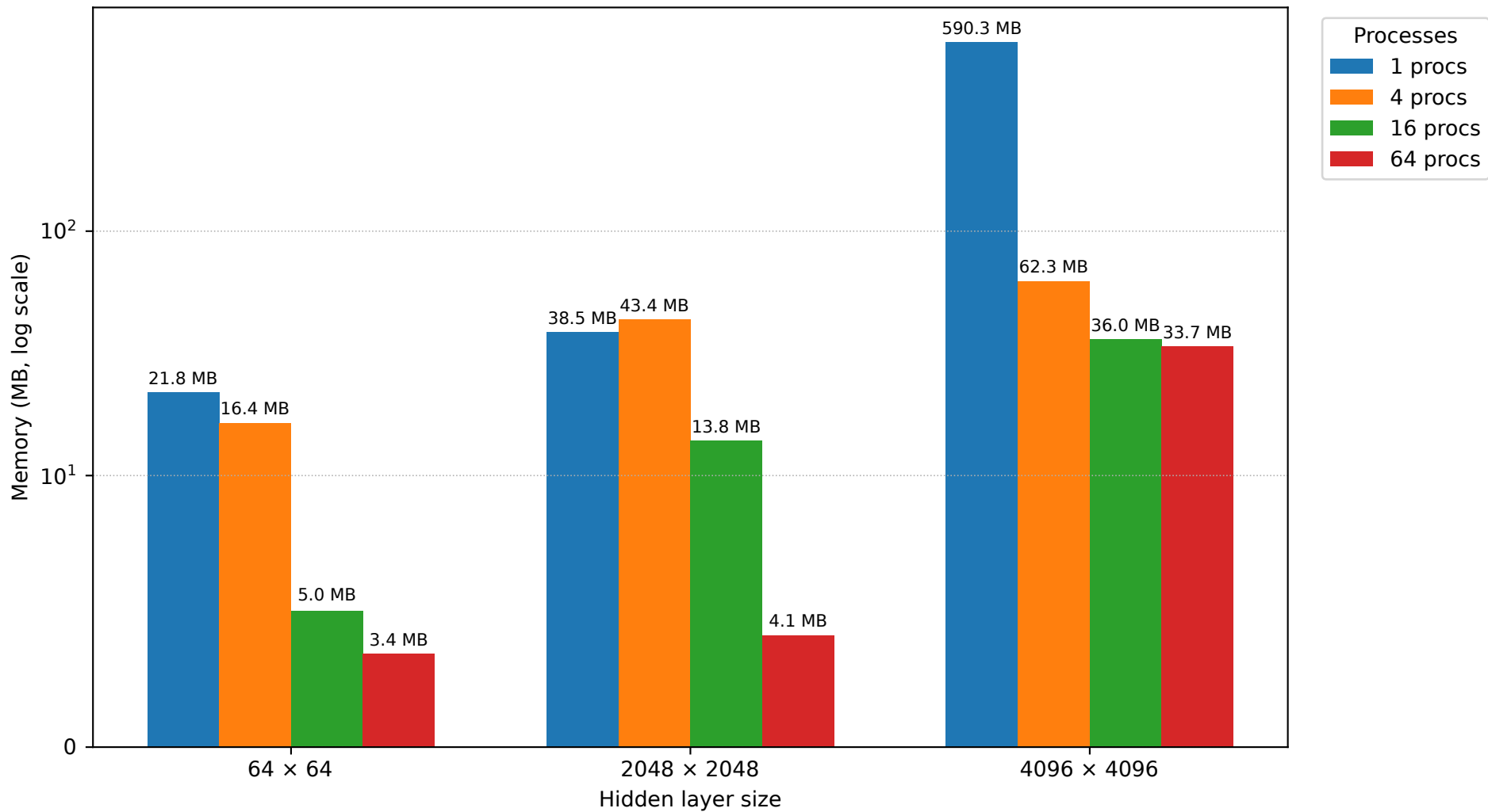
Mean Per Process Memory Increase Batches Per Epoch: 60, Batch Size: 1,000
