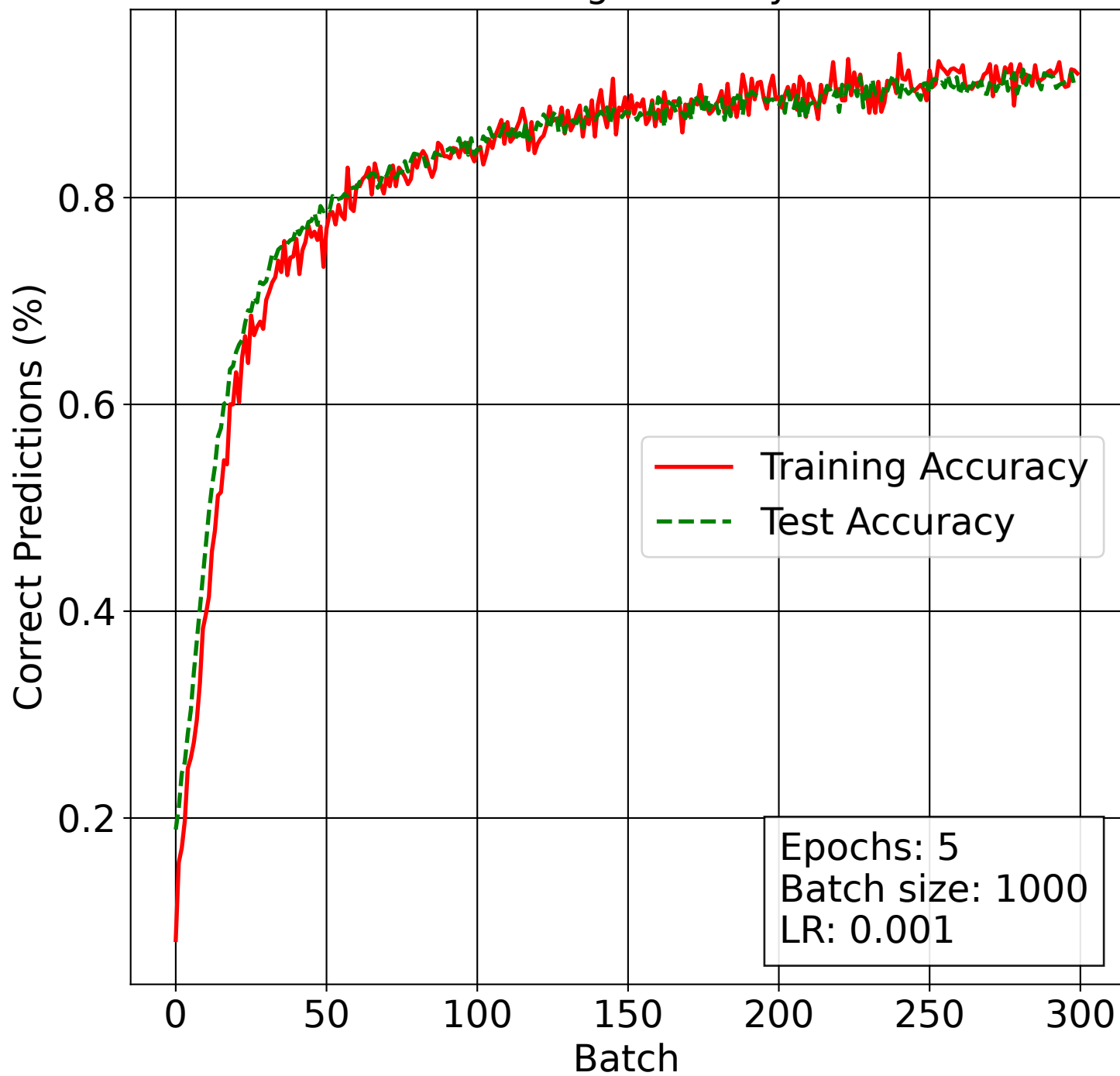
Training Accuracy
