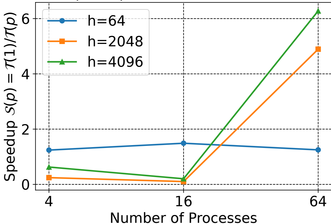
Speedup vs Number of Processes
