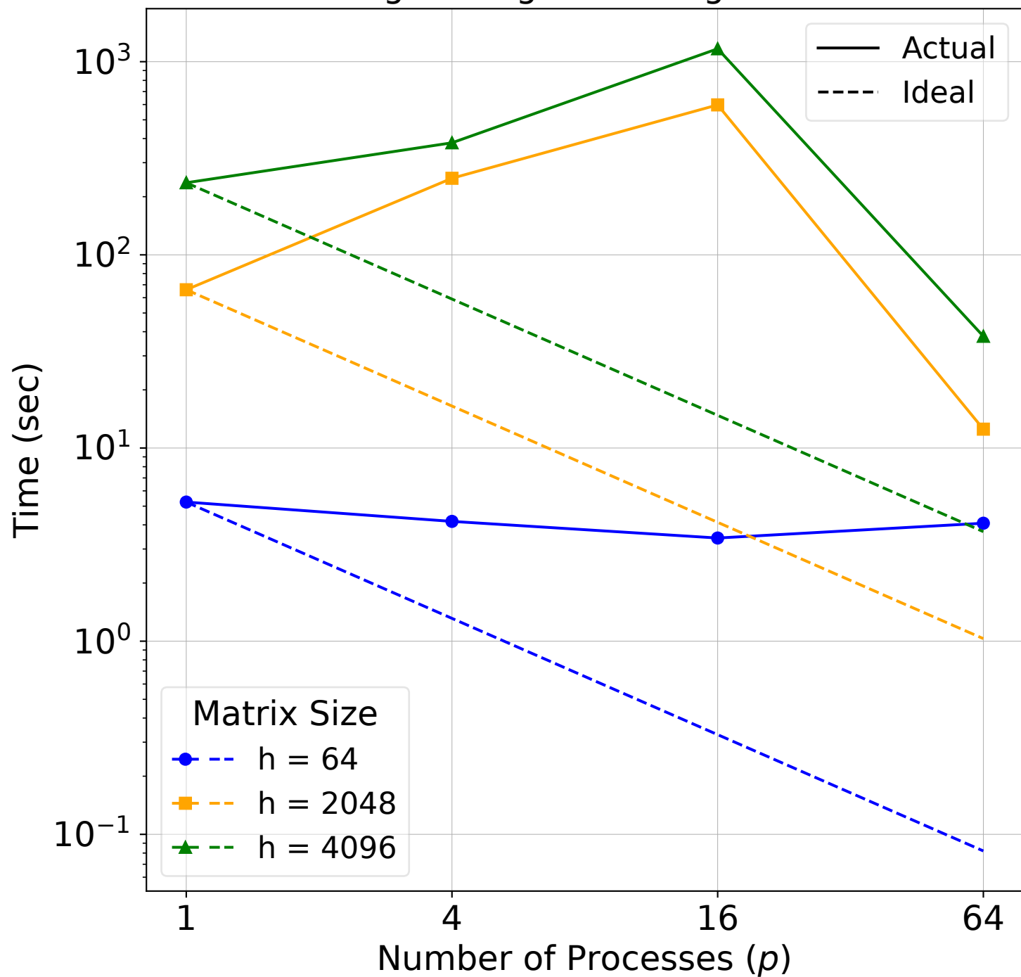
Strong Scaling of Training Runtime
