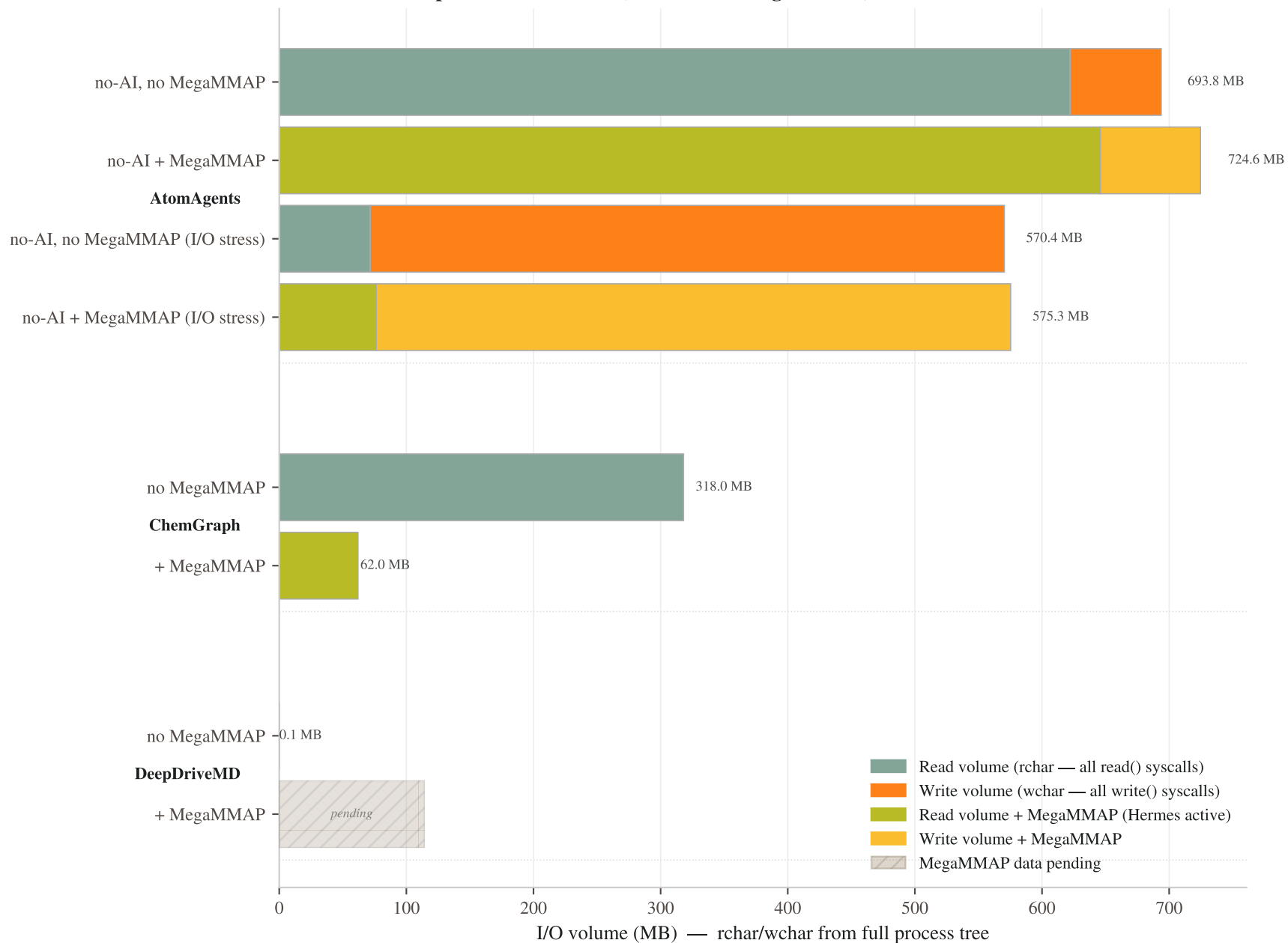
Data Movement per Workflow Run (Baseline vs. MegaMMAP)
