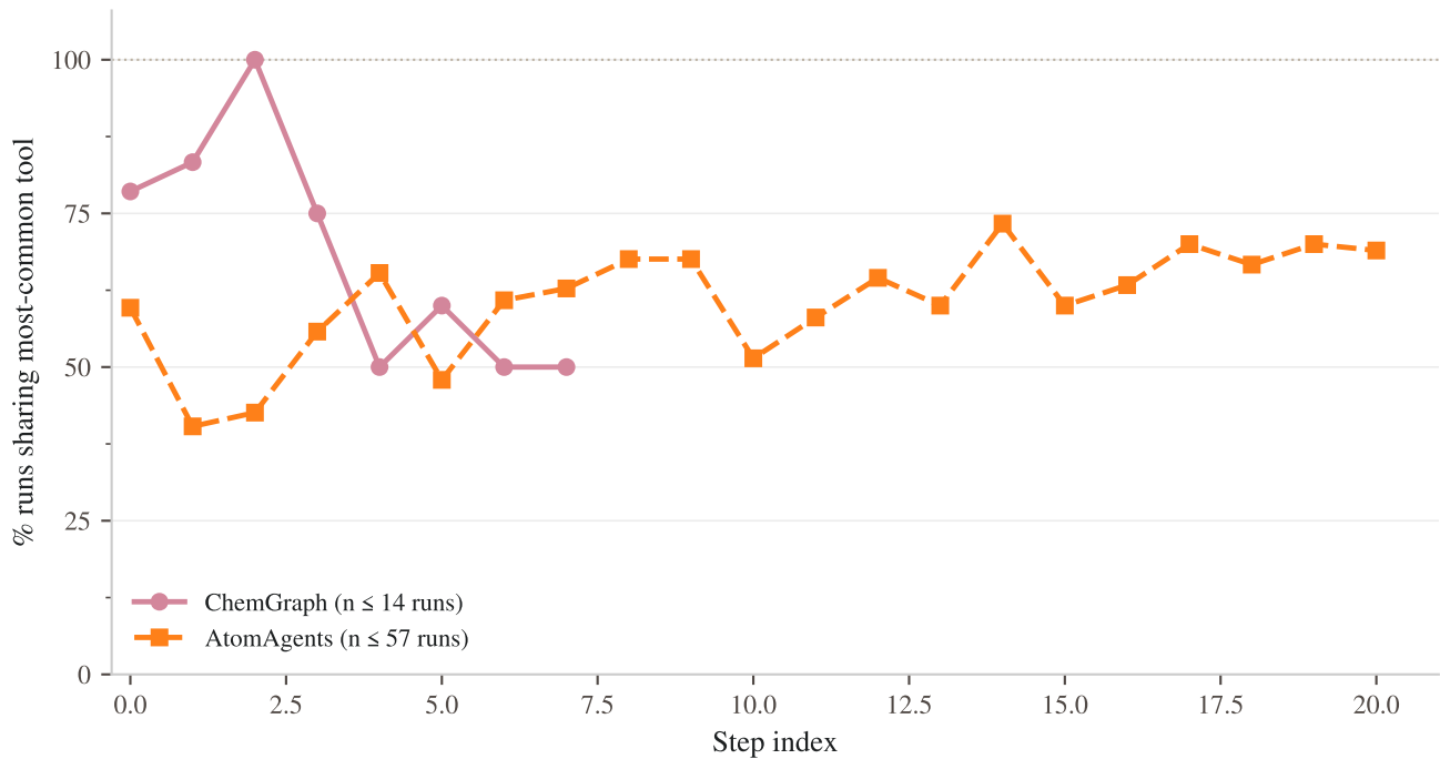
Workflow Consistency Across Runs
