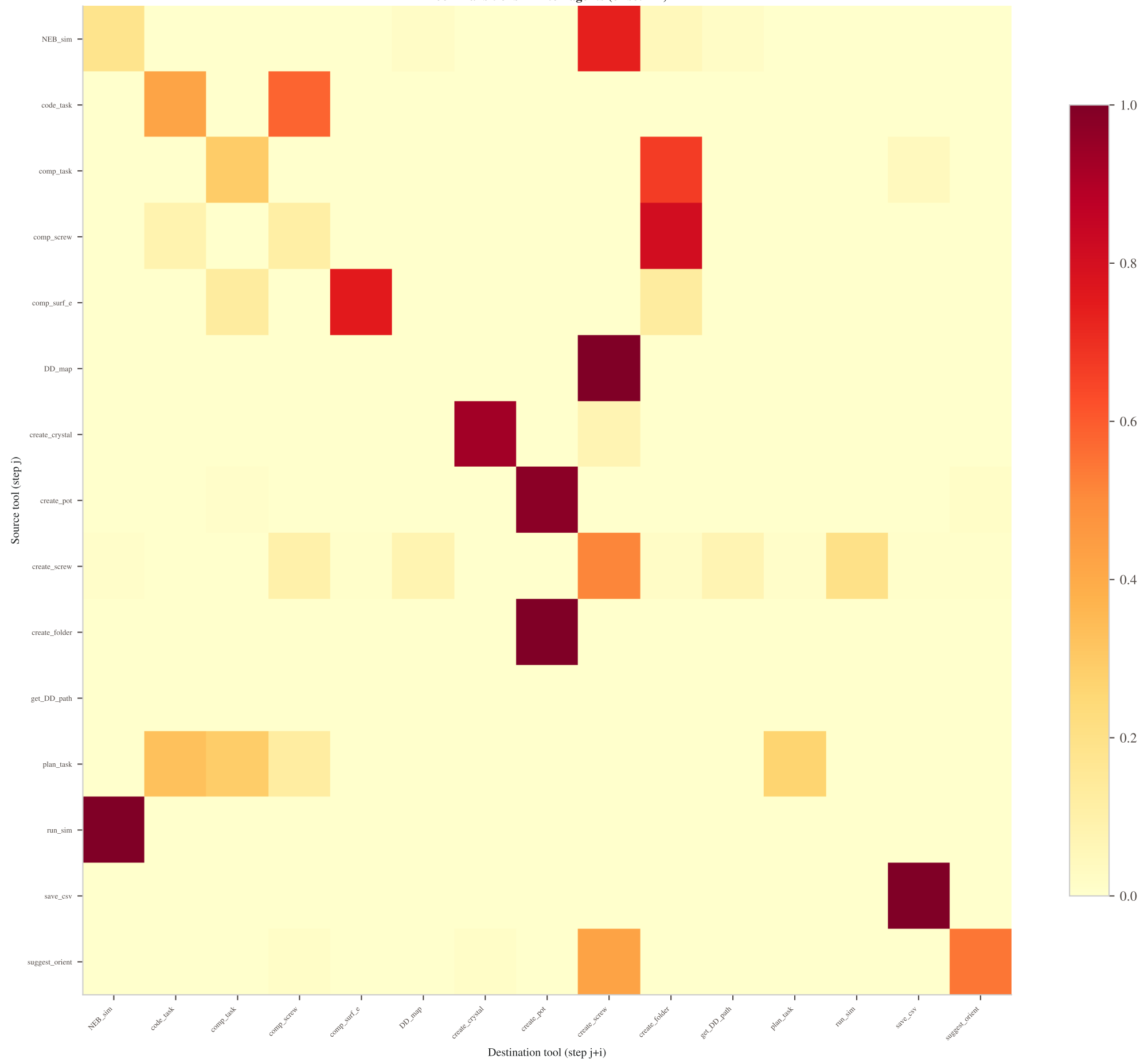
Tool Transitions — Atomagents (offset i=1)
