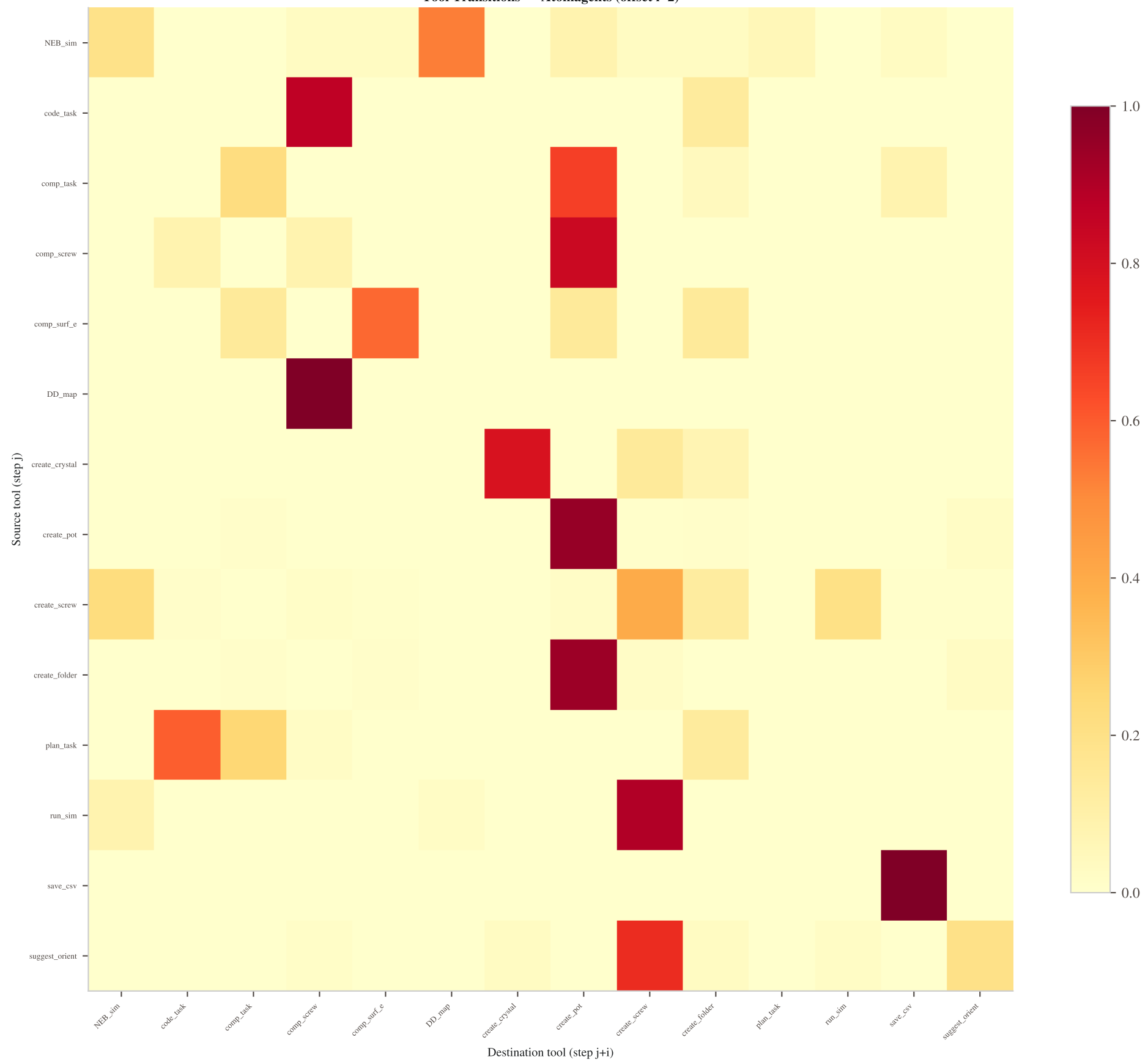
Tool Transitions — Atomagents (offset i=2)
