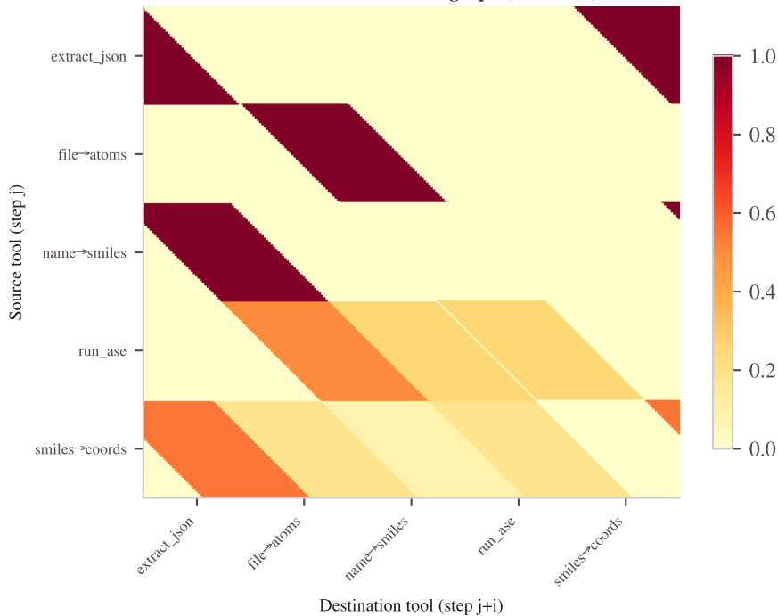
Tool Transitions — Chemgraph (offset i=2)
