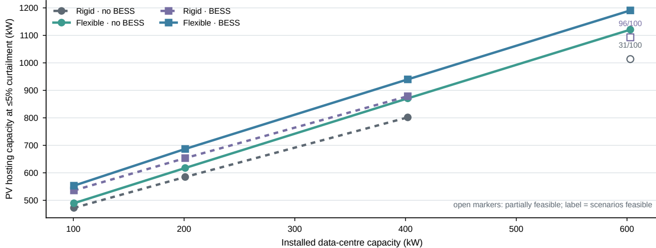
a Workload flexibility shifts the joint DC-PV feasibility boundary
