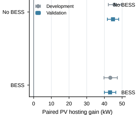
b Gain at a 201-kW data centre
