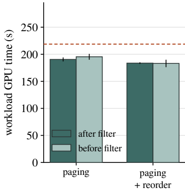
TPC-H SF100
