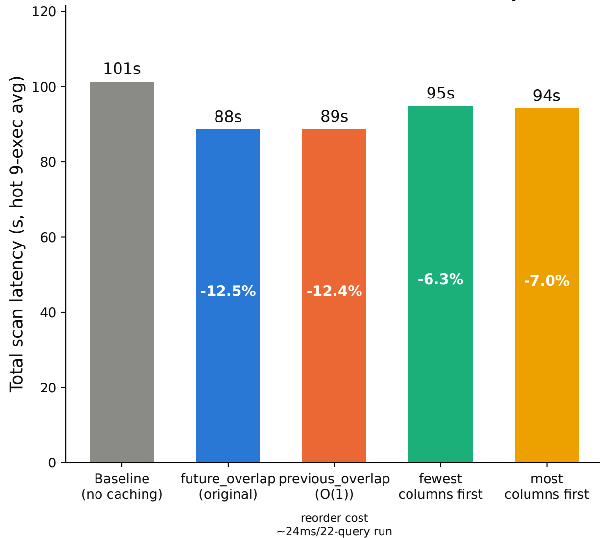
Online resident-aware reorder: scan latency
