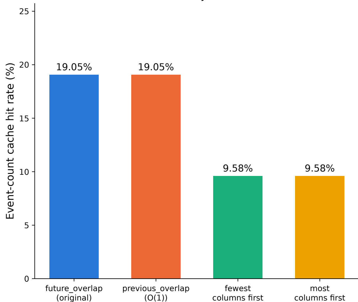
Cache hit rate by tiebreak rule
