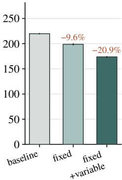
TPC-H SF100
