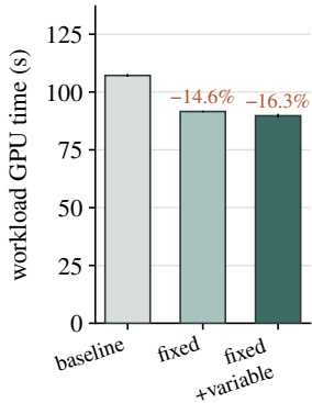
TPC-H SF50
