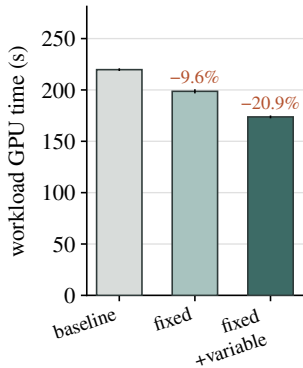
TPC-H SF100
